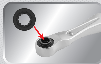
▪ D-head 12 PT design for quick bit replacement
